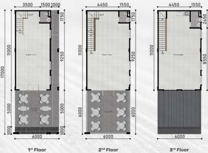
6x17 Corner - 3 Floors
