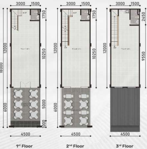
4,5x18 3 Floors
