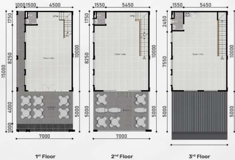
7x15 Corner - 3 Floors
