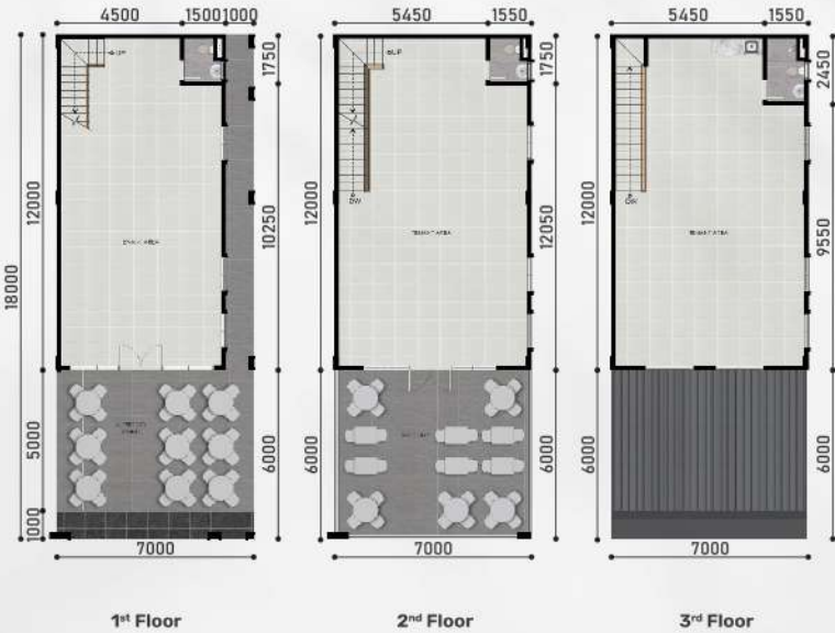
7x18 Corner - 3 Floors
