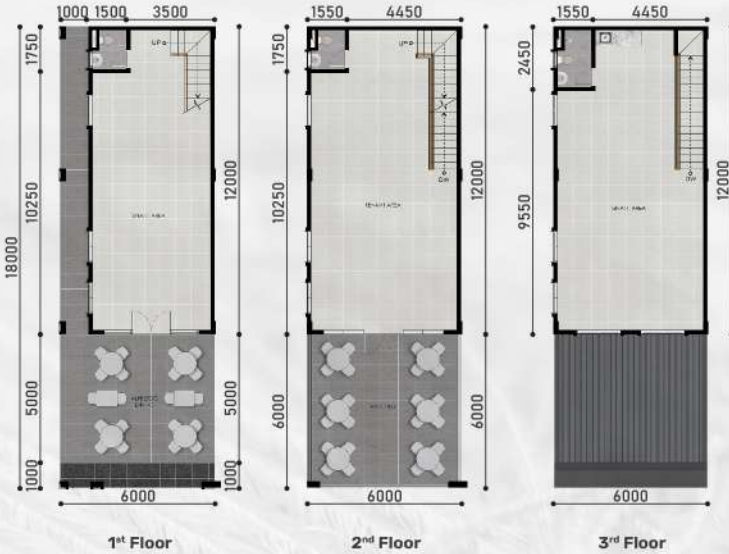
6x18 Corner - 3 Floors
